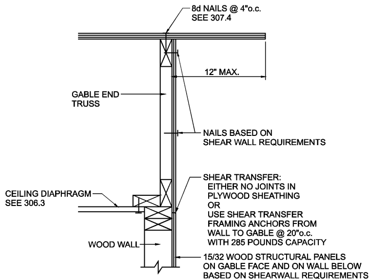
FIGURE 305K GABLE ENDWALL, PLATFORM FRAMING ALTERNATE METHOD
