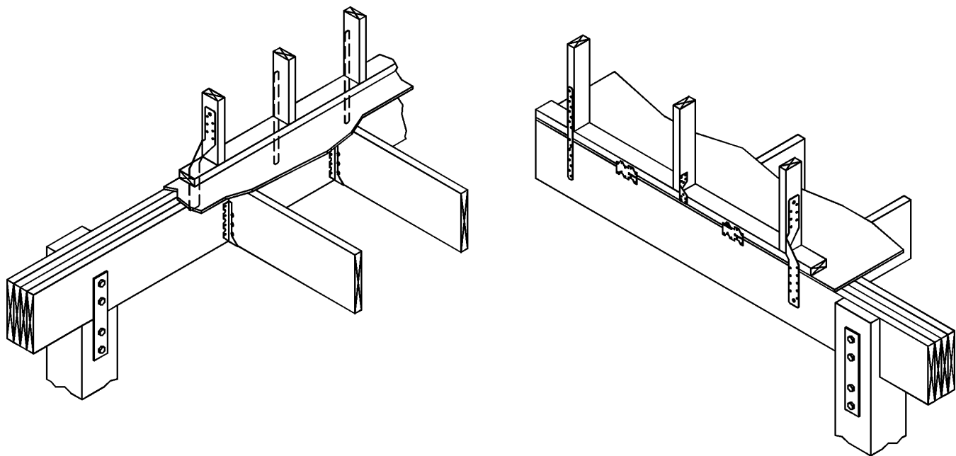
FIGURE 303J FLOOR JOIST TO GIRDER CONNECTIONS
